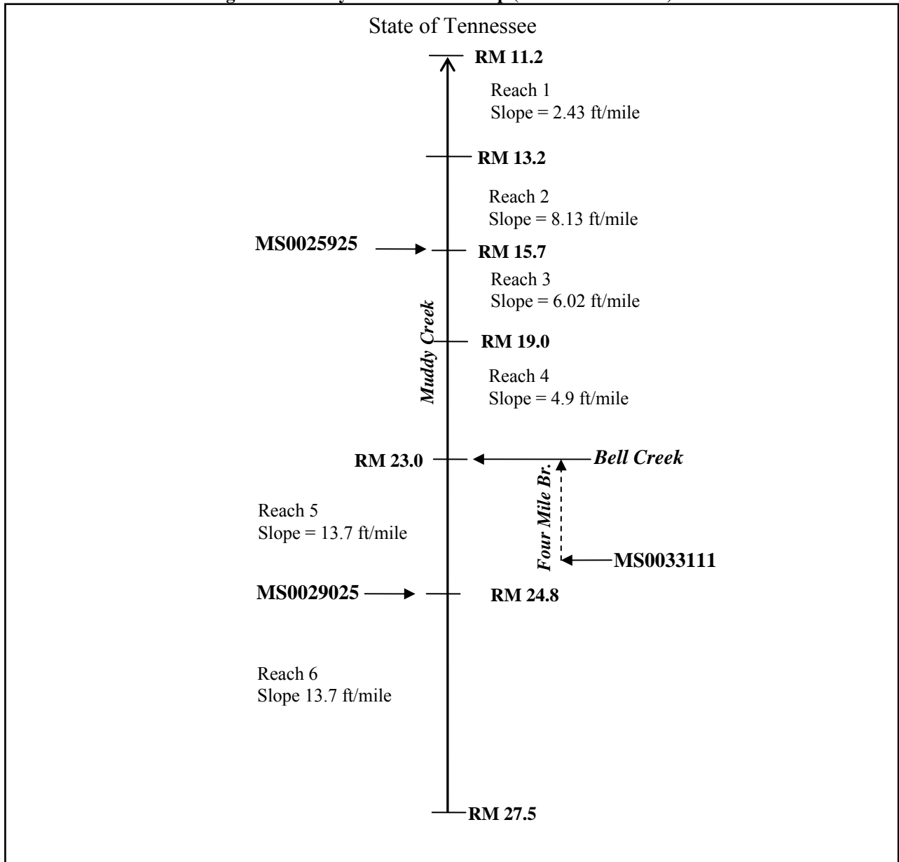
Figure 8. Muddy Creek Model Setup (Note: Not to Scale)
