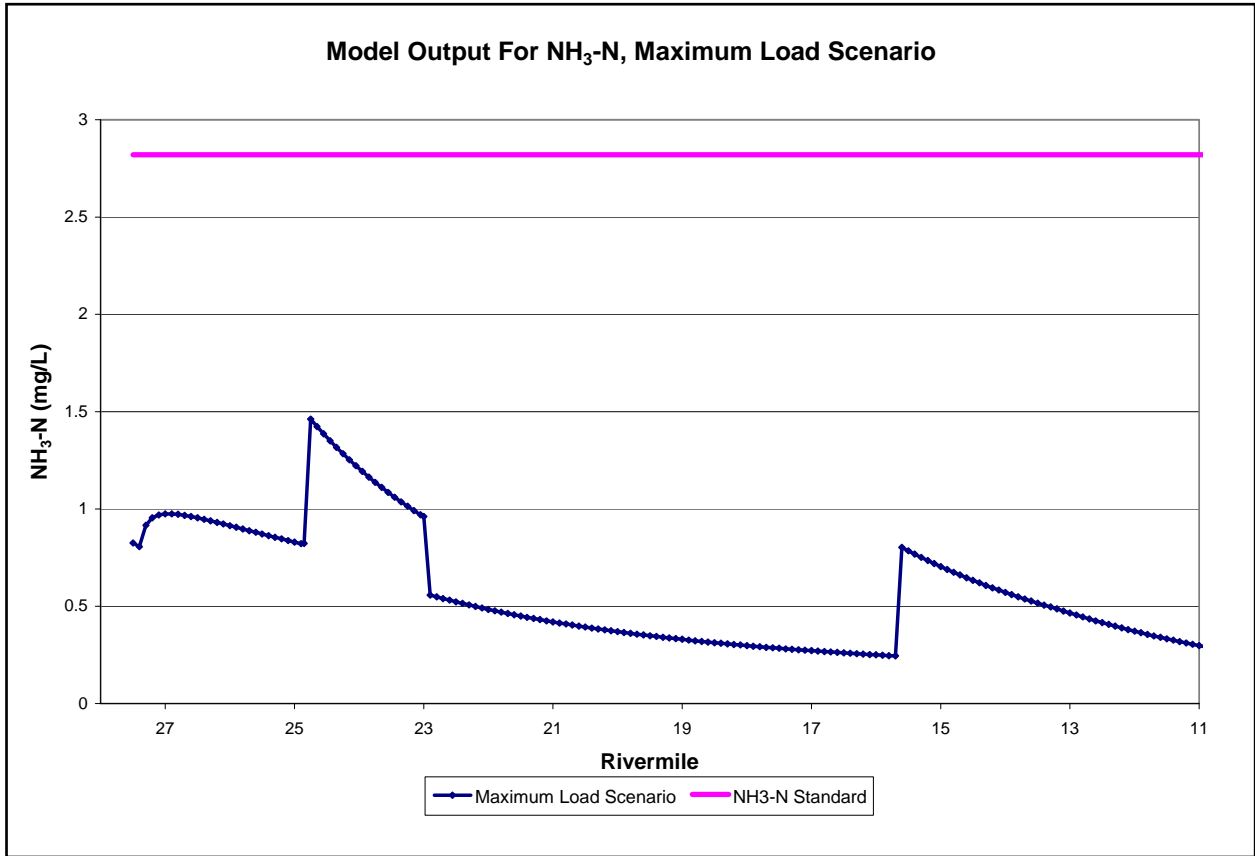
Figure 12. Model Output for NH 3 -N in the Muddy Creek, Maximum Load Scenario
