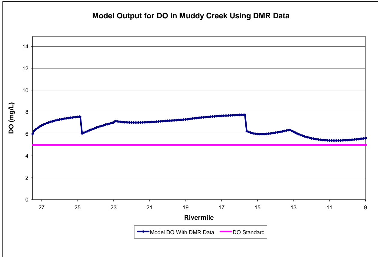
Figure 10. Modeled DO at 7Q10 Conditions with DMR Data
