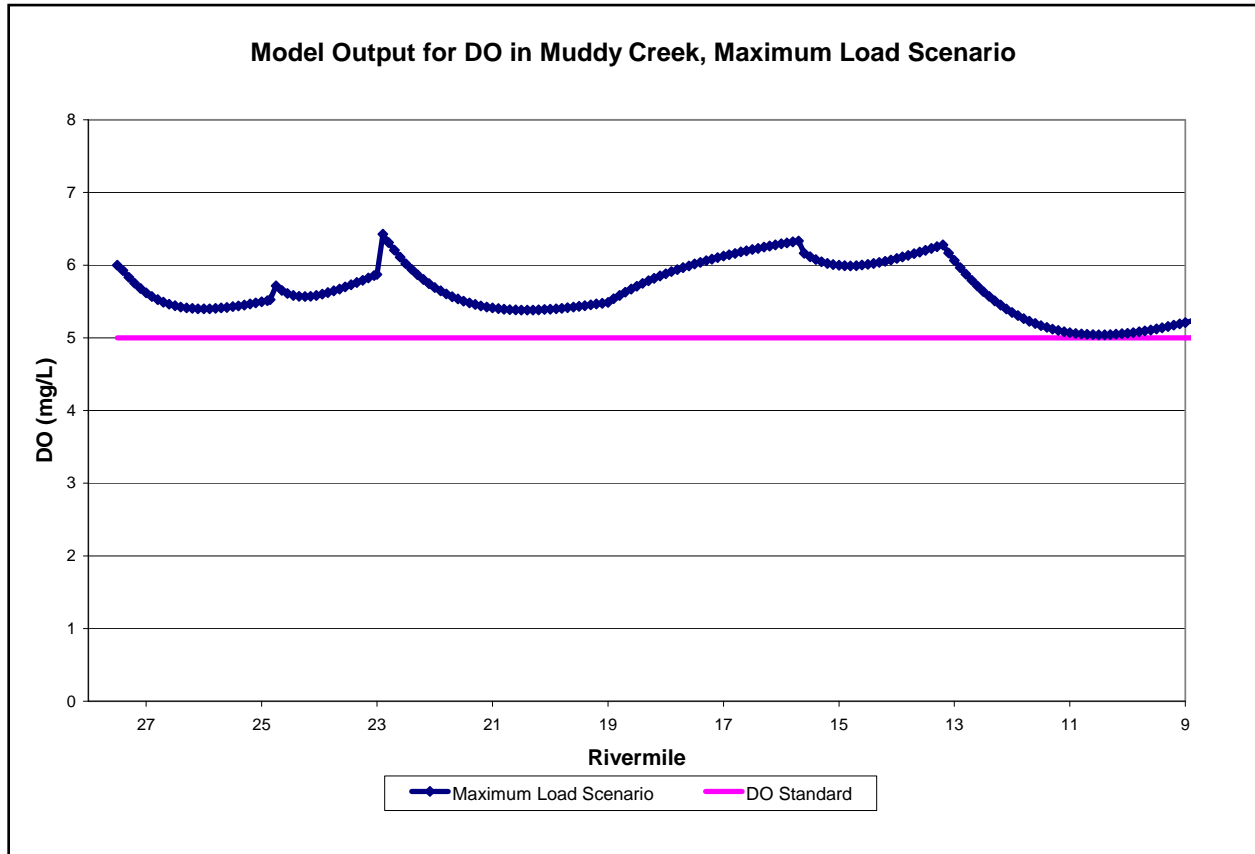
Figure 11. Model Output for the Muddy Creek for DO, Maximum Load Scenario
