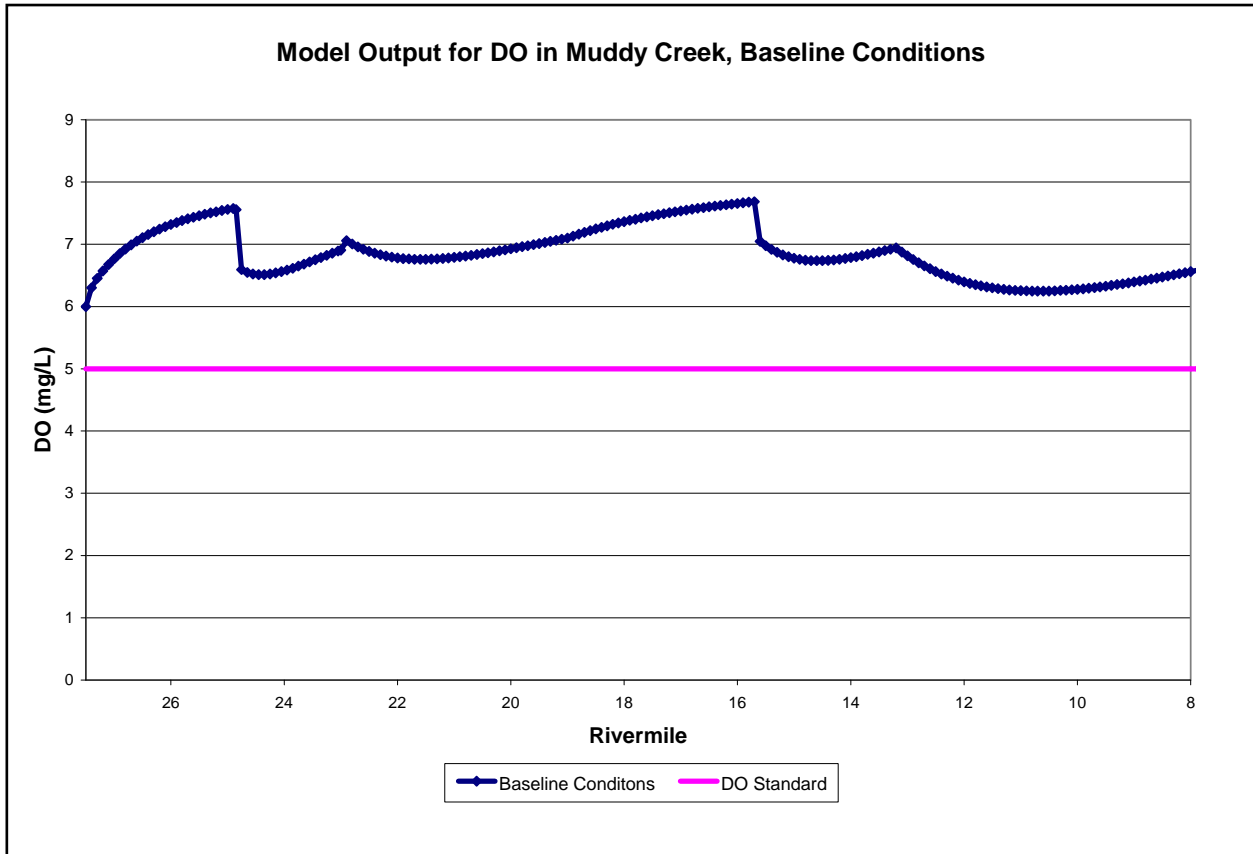
Figure 9. Model Output for the Muddy Creek for DO, Baseline Conditions
